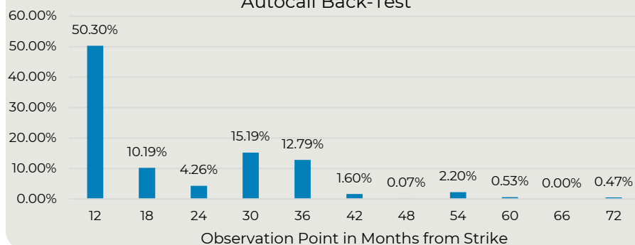
Autocall Back-Test
