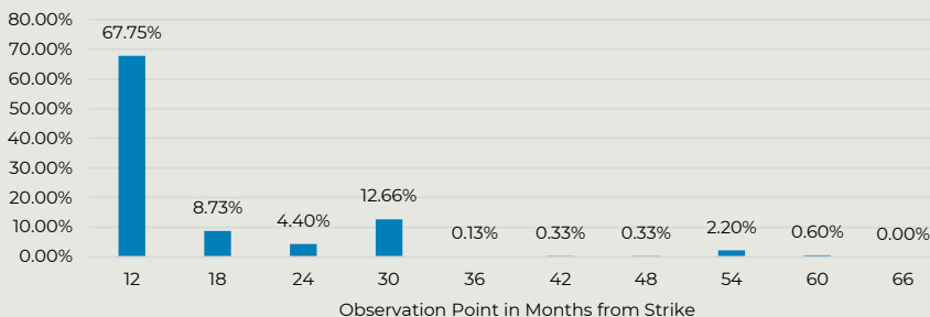
Autocall Back-Test
