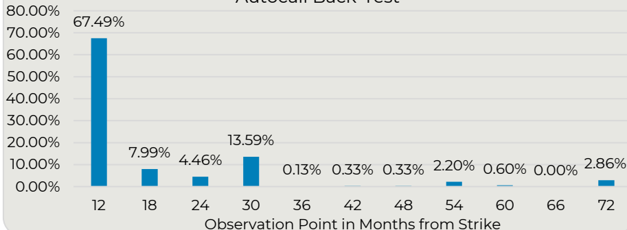
Autocall Back-Test
