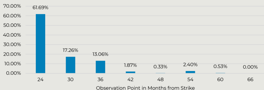
Autocall Back-Test
