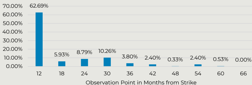
Autocall Back-Test
