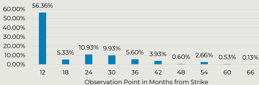
Autocall Back-Test
