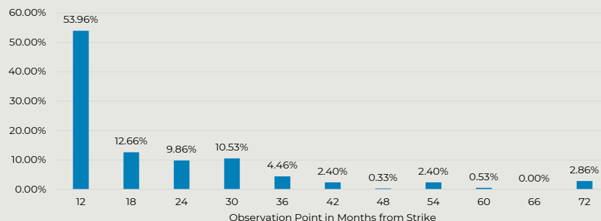
Autocall Back-Test
