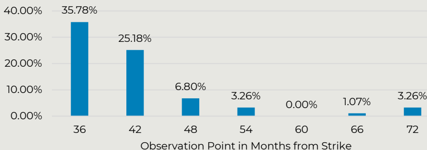
Autocall Back-Test
