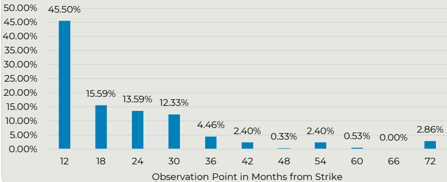
Autocall Back-Test
