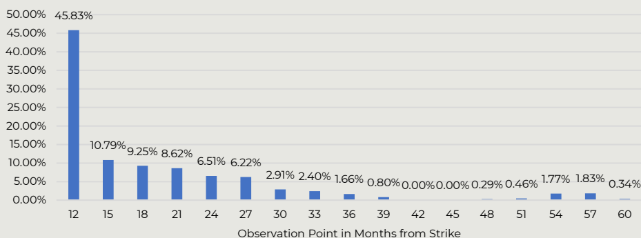
Autocall Back-Test
