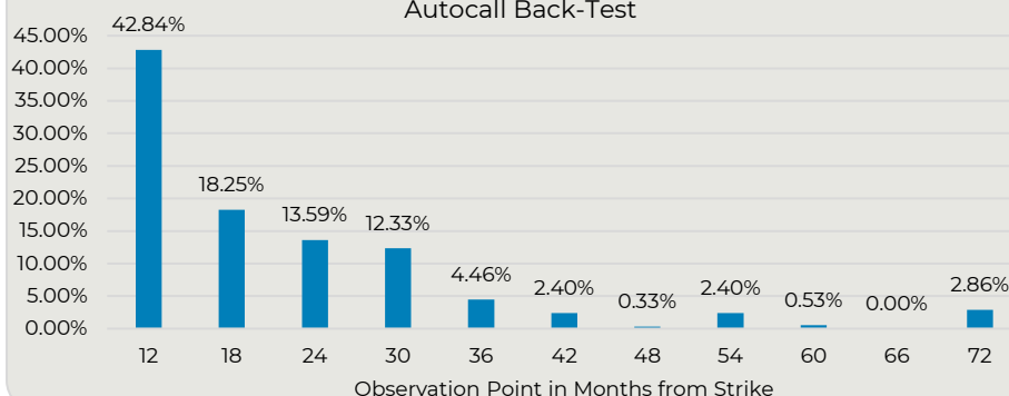
Autocall Back-Test
