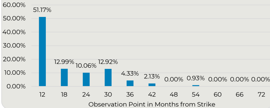
Autocall Back-Test
