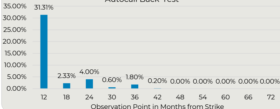
Autocall Back-Test
