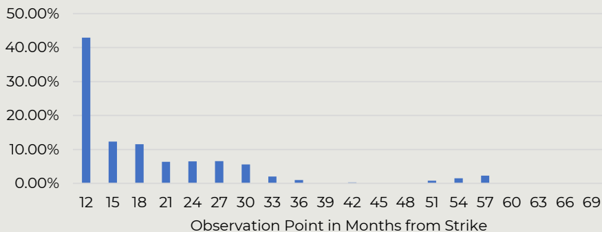
Autocall Back-Test
