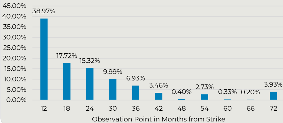
Autocall Back-Test
