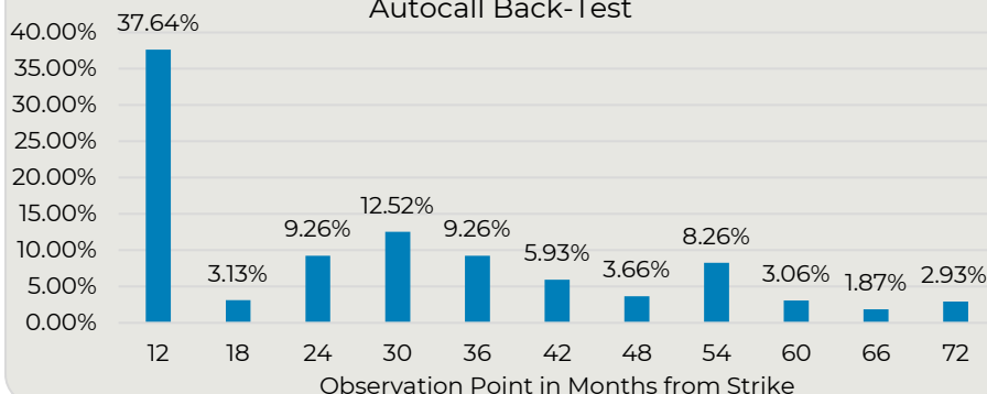
Autocall Back-Test
