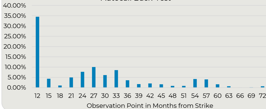
Autocall Back-Test
