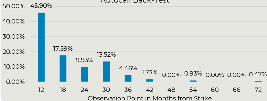
Autocall Back-Test
