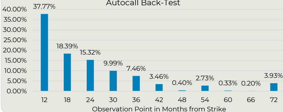
Autocall Back-Test
